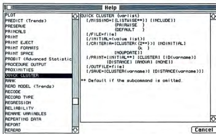
Help with SPSS: the left window lists all the SPSS commands, and the right window lists all possible parameters for each command.
