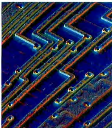
A section of the data memory controller area of the Mac 68040 chip at approximately 1500x magnification, photographed and colorized with David Scharf's Scanning Electron Microscope Multi-Detector Color Synthesizing System, and saved as a TIFF file.
