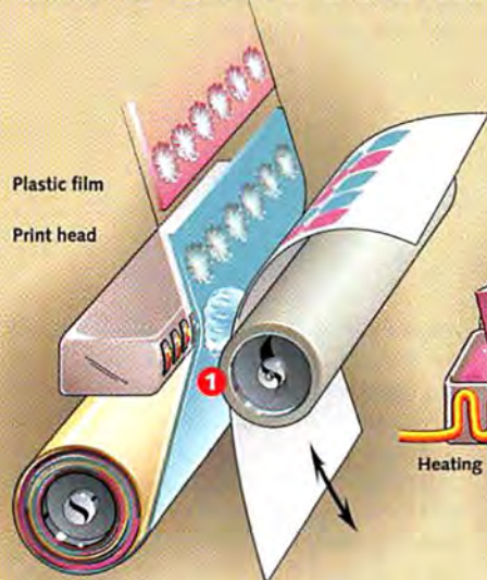
Dye Sublimation
