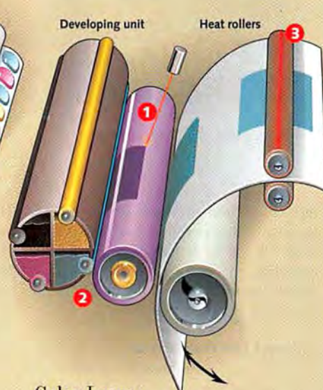
Color Laser
