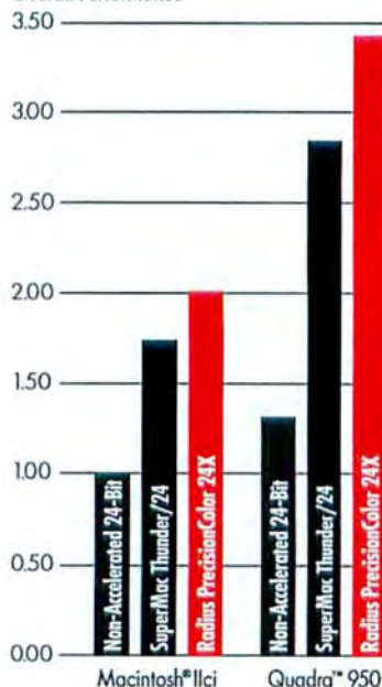
Hydra QuickDraw Performance Test Overall Performance
