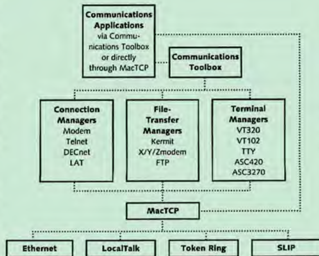
Help from Apple The Communications Toolbox and MacTCP work together to provide a base for other communications applications.
