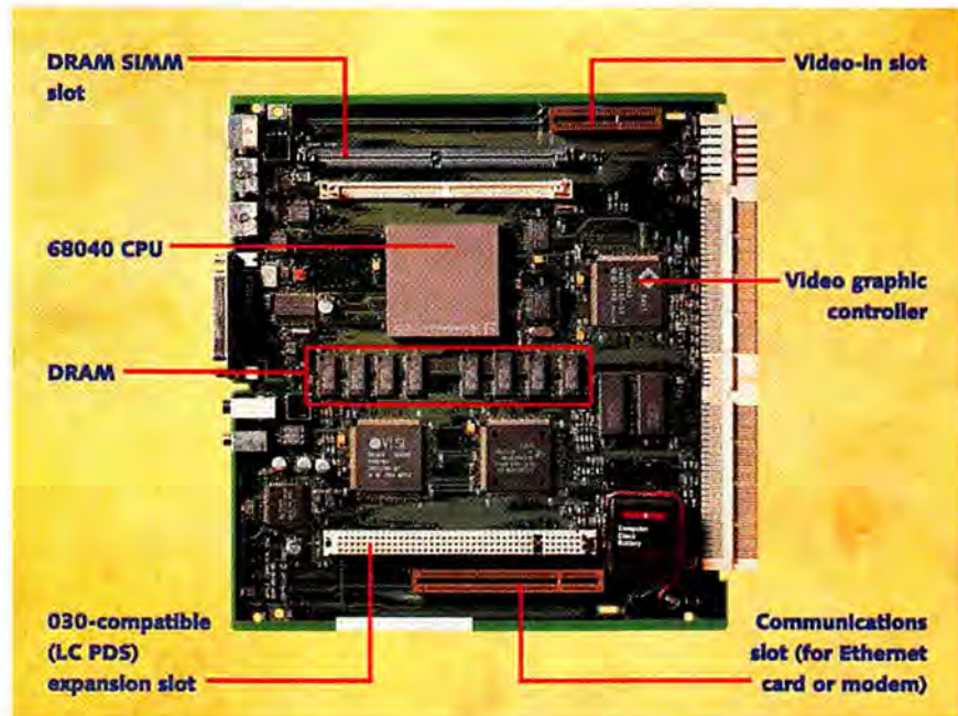
The 630 Family Logic Board The tray-mounted logic board of the 630 series makes maintenance relatively convenient. The only differences between the various 630 models lie in the CPU—a full 68040 for the Quadra 630 compared with a 68LC040 (which lacks an FPU) for all other units. The various 630 machines come with 4MB to 8MB of RAM standard, and all are expandable to 36MB.
