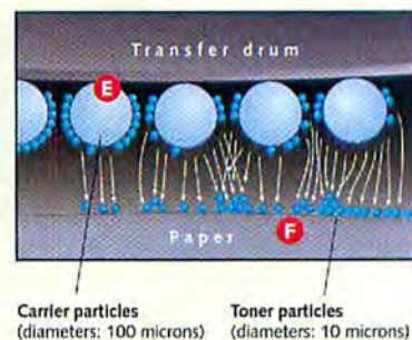
Dual-component toner (mechanism not shown)
