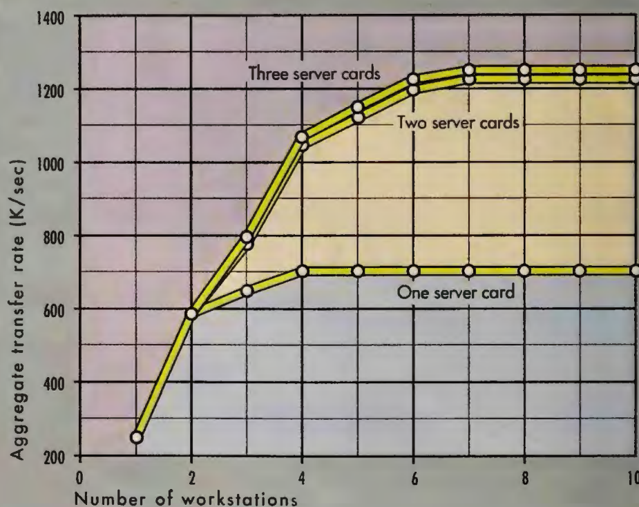
FIGURE 1: A 20-MHz server running NetWare 3.0 was tested with Novell's Perform2 utility and NE2000 ethernet cards. Two cards nearly double the aggregate transfer rate.
