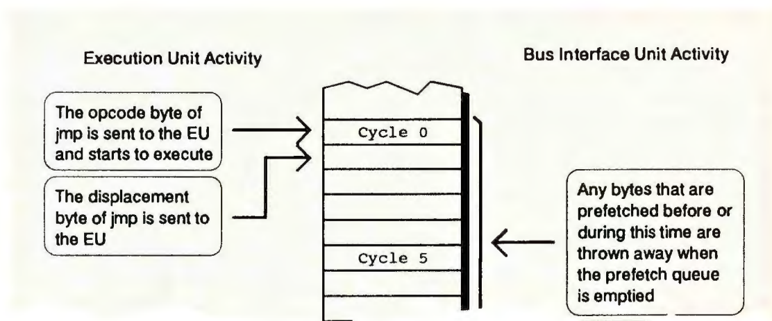
A figure from " Zen of Assembly Language " shows how you can speed a program by fetching one instruction while another is executing.
